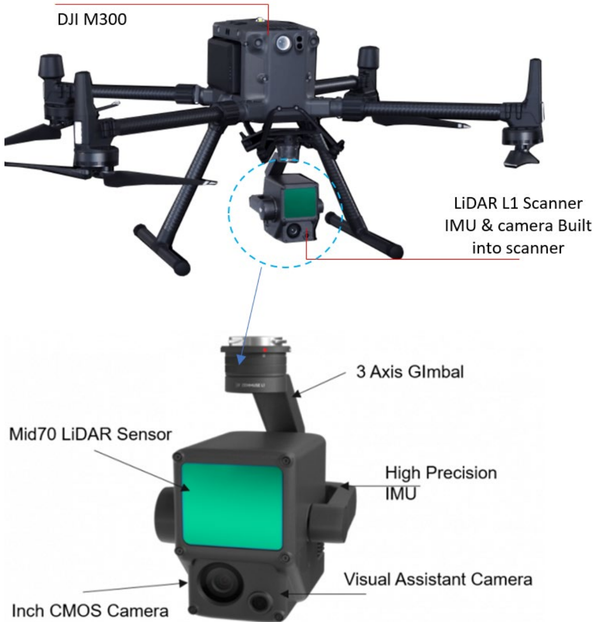
Figure 7 Multi Rotor DJI M300 with L1 Laser Scanner 7
