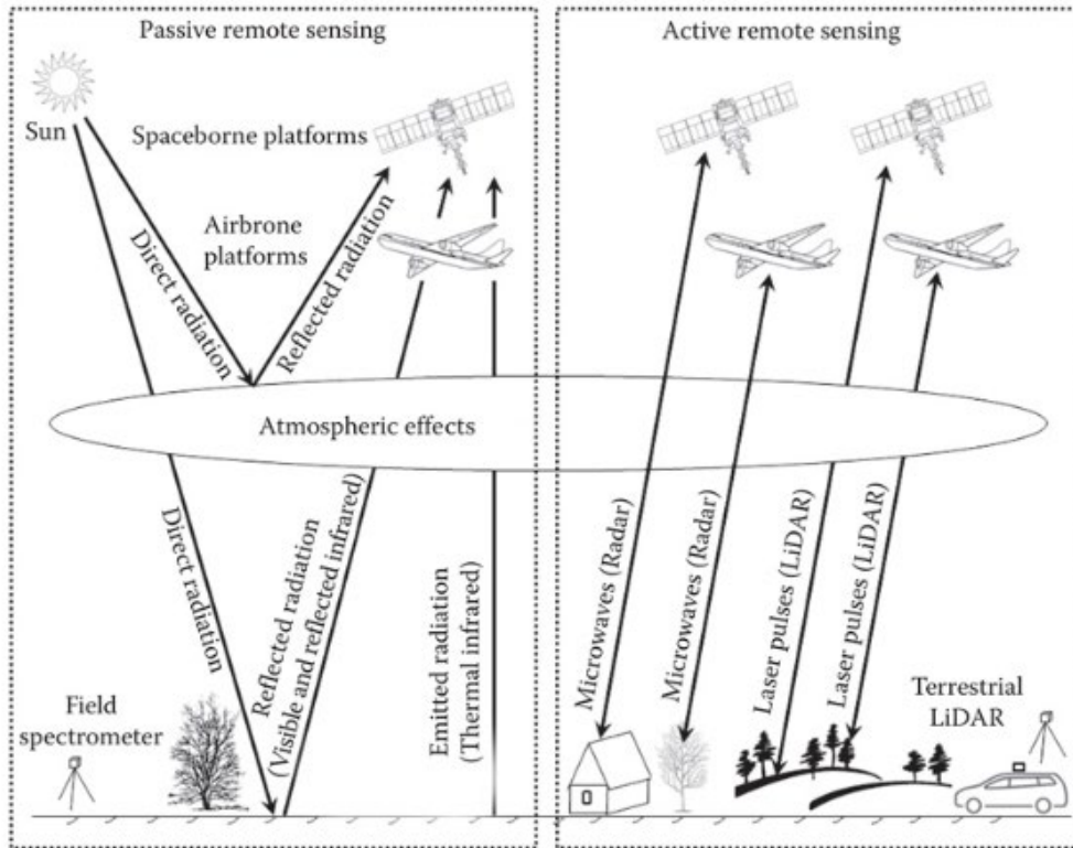
Figure 2 Passive and Active remote sensing 8
