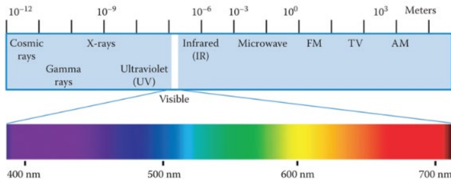
Figure 5 Electromagnetic spectrum 3
