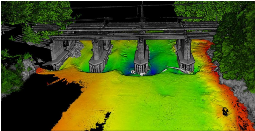
Figure 19 Example a River Eden LiDAR scan 14
