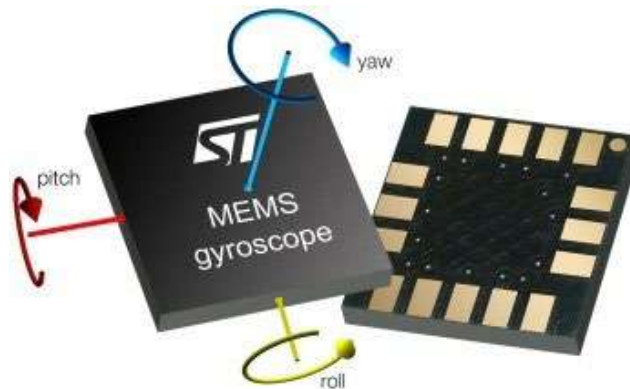
Figure 16 Gyroscope MEMS (STmicroelectronics)
