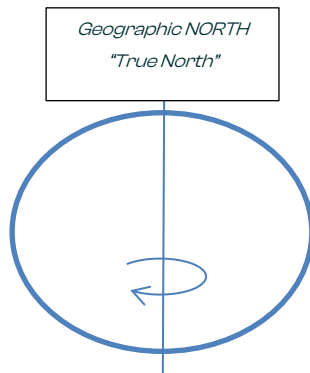
Figure 2-2 rotation axis = geographic North (right)
