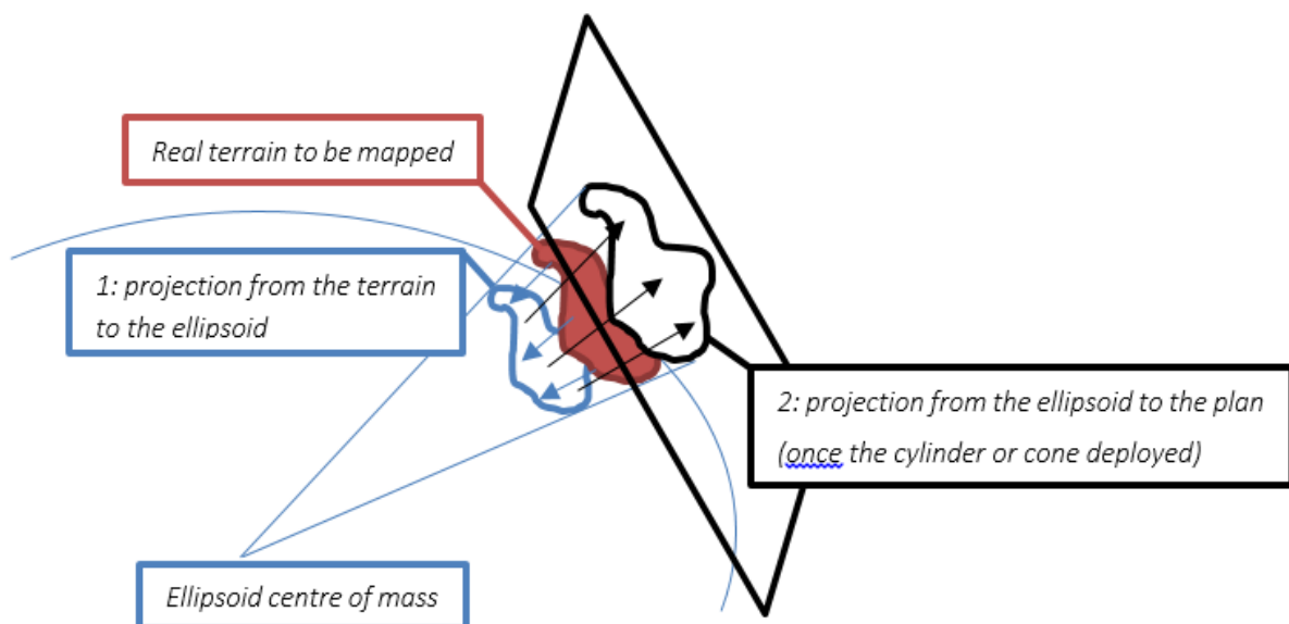
Figure 4-1 The two successive projections to obtain a map
