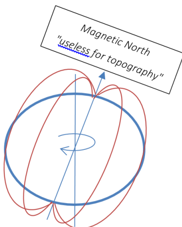
Figure 2-3 magnetic field declination in 2015 (nceinoaa.gov)
