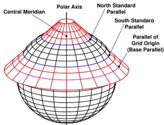
Figure 4-17 Lambert secant projection (researchgate.com)
