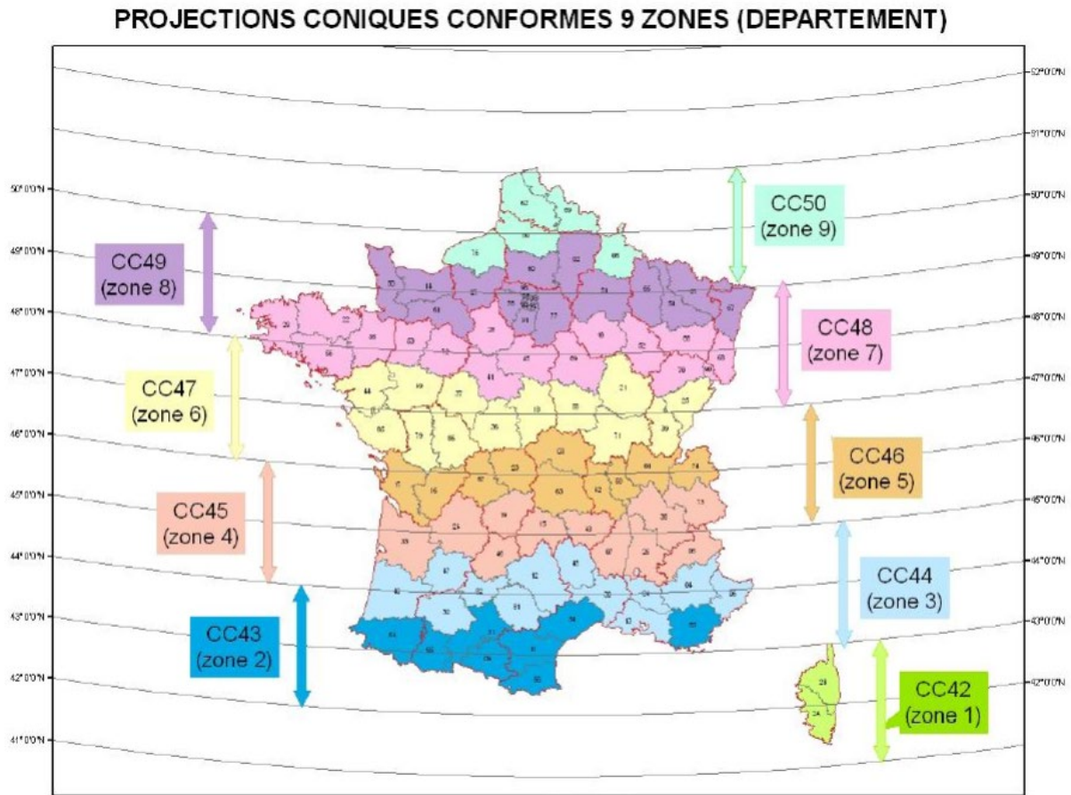
Figure 4-24 the 9 zones of RGF93-CC 9 zones projections (IGN)
