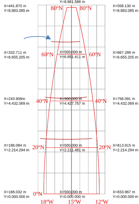
Figure 4-12 coordinates in a UTM strip
