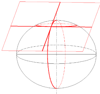
Figure 4-7 Azimuthal tangent representation
