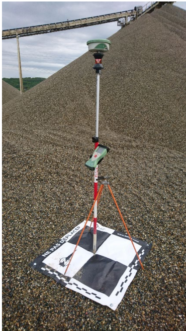
Figure 7-2 GNSS measure on a target (Chivas)
