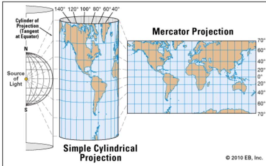
Figure 4-8 direct Mercator projection (Britanica.com)
