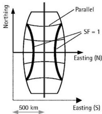
Figure 4-15 scale factor=1 along standard meridians (what-when-how.com)
