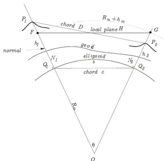
Figure 4-14 distance projection from field to ellipsoid
