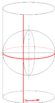
Figure 4-3 direct cylindrical projection
