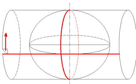
Figure 4-4 transverse cylindrical projection
