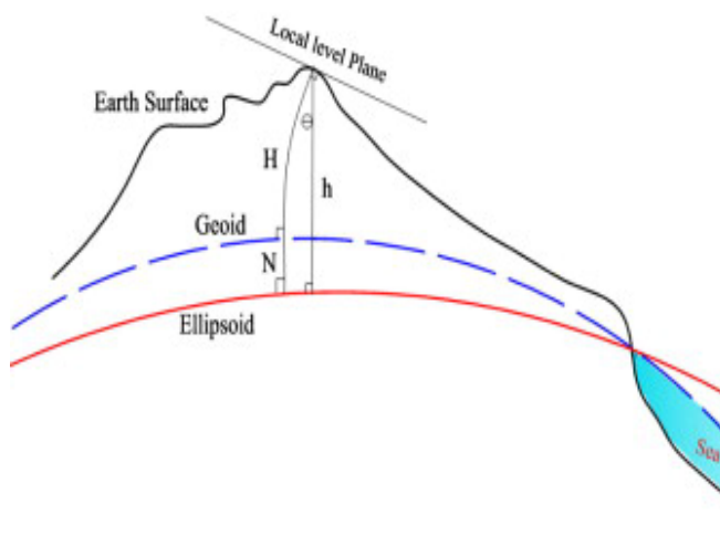
Figure 5-4 heights measurements (USGS)
