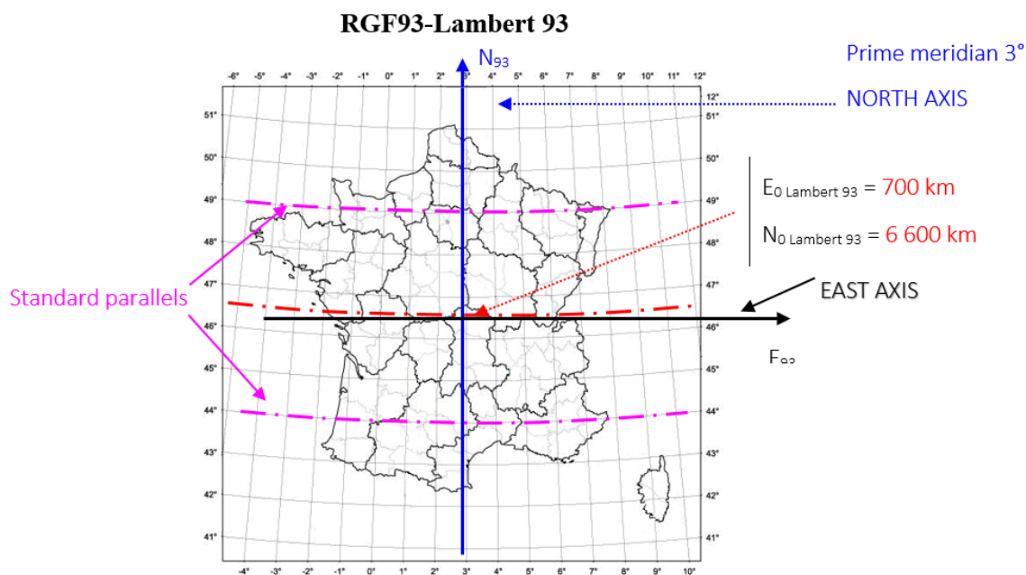
Figure 4-20 axis of the RGF93-Lambert93 projection system
