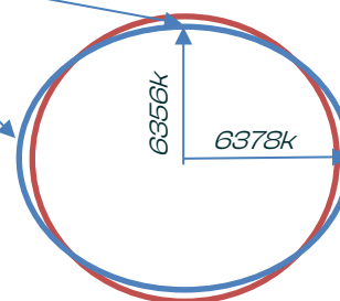
Figure 2-1 WGS84 ellipsoid
