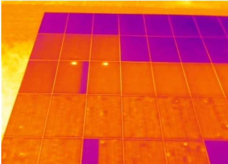
Figure 2-12 Numerous simultaneous defects ( diagnosticphotovoltaique.fr )
