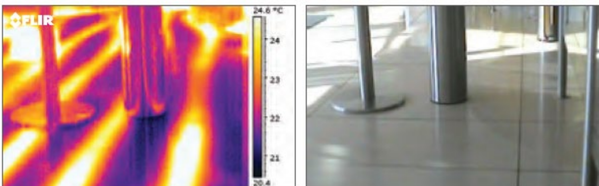
Figure 2-4: Localization of the heating system (FLIR Systems)
