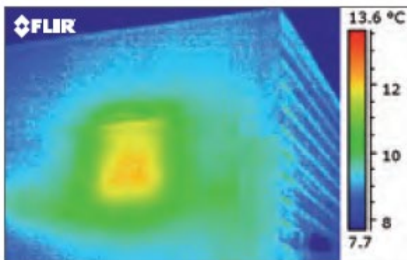
Figure 2-1: Missing insulation in the facade (FLIR Systems)
